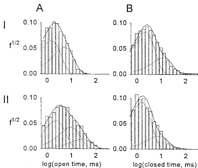
FIGURE 6 Effect of 1 mM cis DTNB on open and closed time distributions for a single RyR MH . Open and closed times are collected into logged bins, and the square root of the relative frequency of events ( f^{1/2} ) is plotted against the logarithm of the open or closed times in ms. (A) Open time distribution. (B) Closed time distribution. In A and B, distributions are shown for control data (I) and during activation by 1 mM cis DTNB (II). The continuous lines in each graph show the multiple exponential function fitted to the data, and the broken lines show the individual exponential components (2 in AI and 3 in each of AII and BII).
