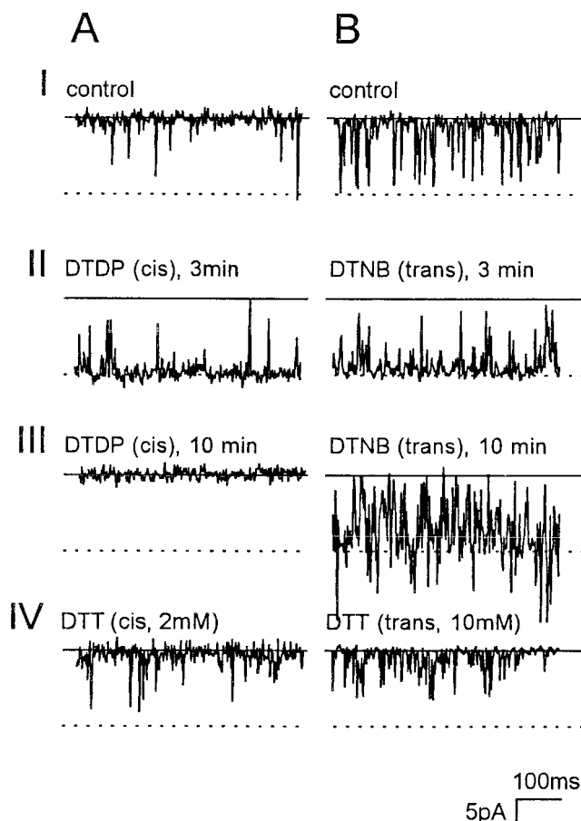
FIGURE 2 Inhibition of normal RyRs by 1 mM cis 4,4'-DTDP, but not by 1 mM trans DTNB. (A) A bilayer containing one RyR channel under control conditions (I), activation 3 min after the addition of 1 mM cis 4,4'-DTDP dissolved in ethanol (II), inhibition 10 min after the addition of 4,4'-DTDP (III), and recovery from inhibition after a final addition of 2 mM DTT (IV). (B) A bilayer containing two normal RyR channels with only one channel active under control conditions (I), increased activity in one channel 3 min after the addition of 1 mM trans DTNB (II), two channels active after a 10-min exposure to trans DTNB (III), and return to control activity in one channel after a final addition of 10 mM DTT (IV). The zero current level is indicated by solid lines, and the maximum open conductance is shown by dotted lines.
